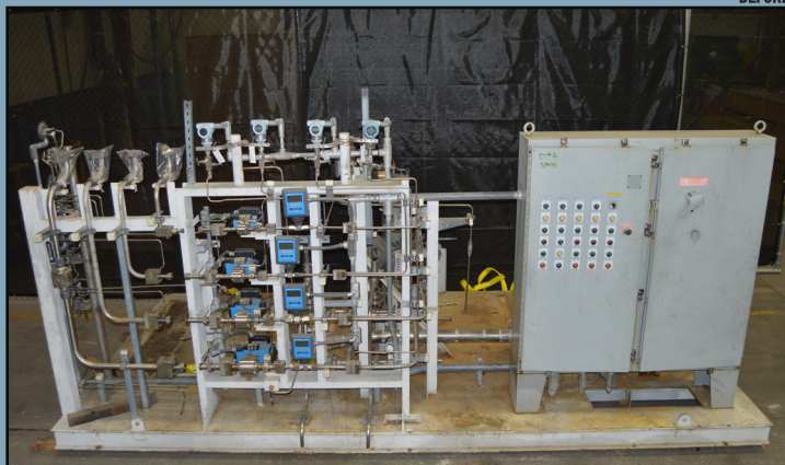
FOGGING SKID UPGRADE UTILIZING CALDWELL ENERGY'S PROPRIETARY CONTROL SYSTEM
