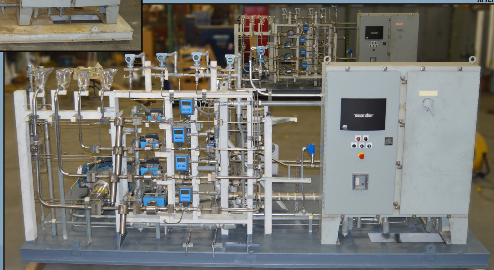
FOGGING SKID UPGRADE UTILIZING CALDWELL ENERGY'S PROPRIETARY CONTROL SYSTEM
